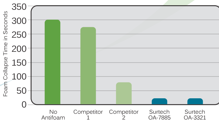
Antifoam Performance in ISO-32 Hydraulic Oil at 100 ppm Actives Level
