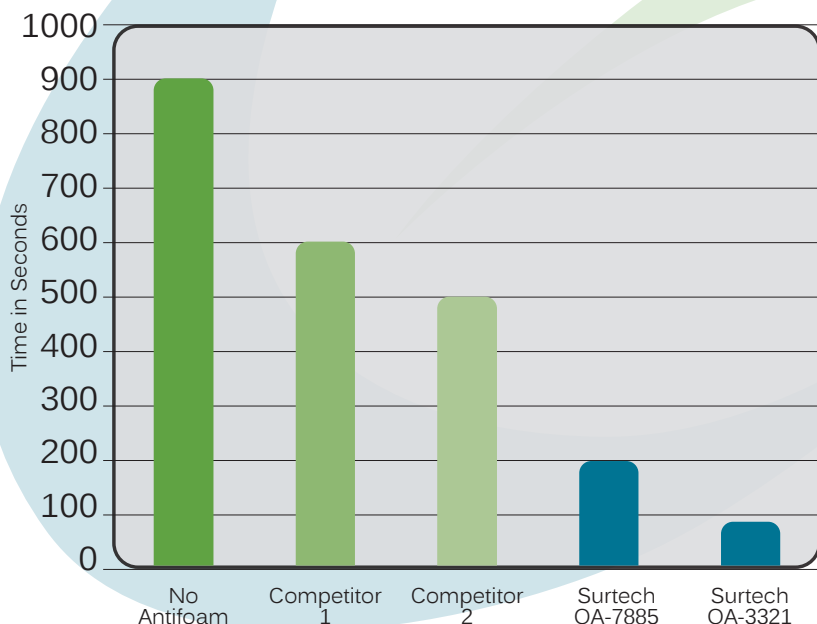
Antifoam Air Release Properties of ISO-32 Hydraulic Oil at 100 ppm Actives Level
